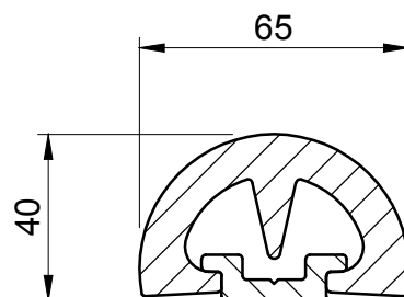
FITTED VIEW ON TRACK PFDBT 4046
