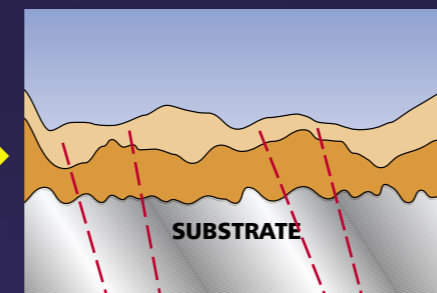
3 Second primer coat fails to achieve required film thickness in places – trouble ahead!
